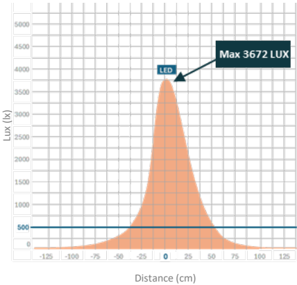
Measurement in lux on the work surface from a side view at 40 cm :
